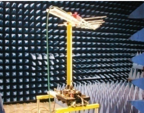
Anechoic Chamber
