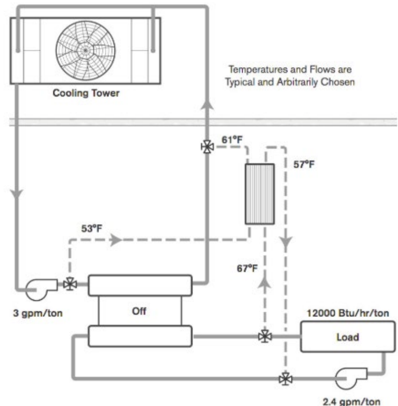
Indirect Free Cooling
